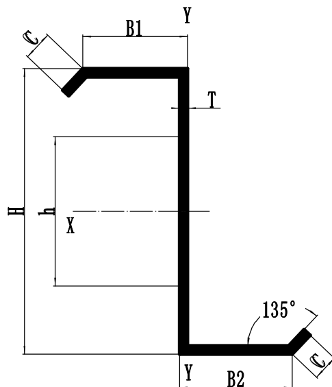
Z型钢 Z-Section Sheet
