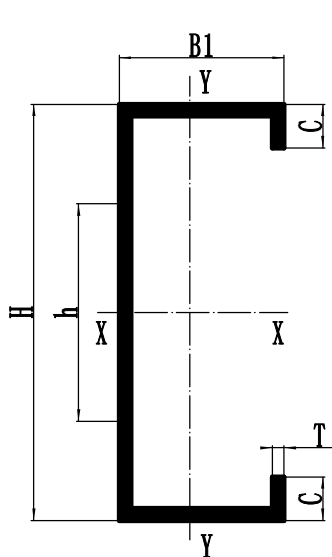
C型钢 C-Section Sheet
